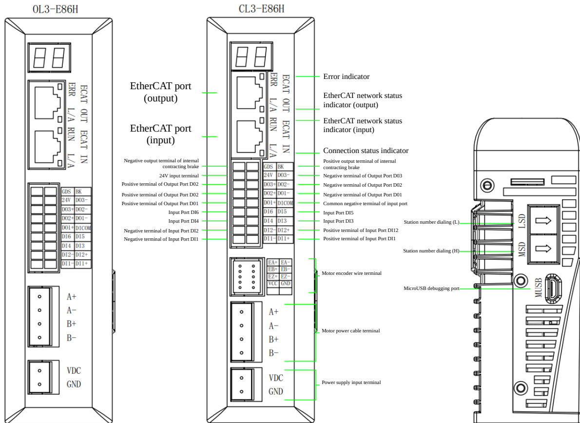
Part description of drive of 86-series
