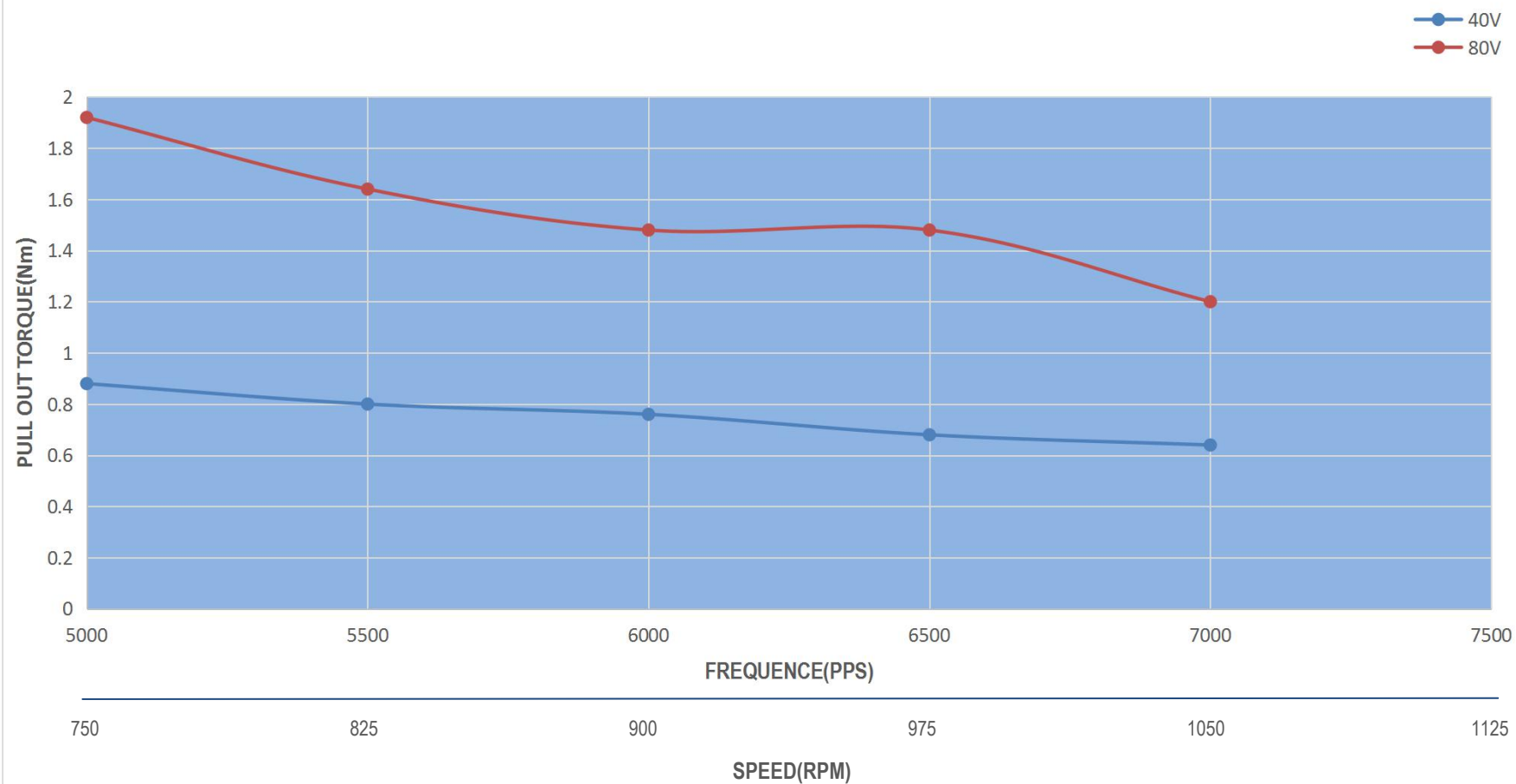
34HS38-3008S PULL OUT TORQUE(5.1A/P 40V/80V HALF STEP)
