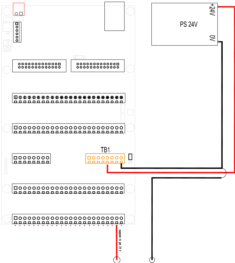
Wiring No.2
