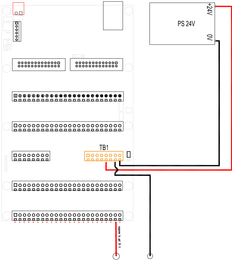
Wiring No.1
