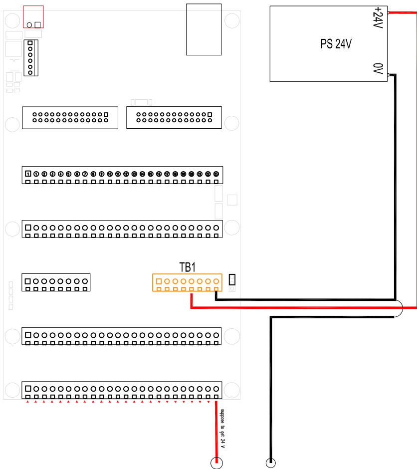
Wiring No.2
