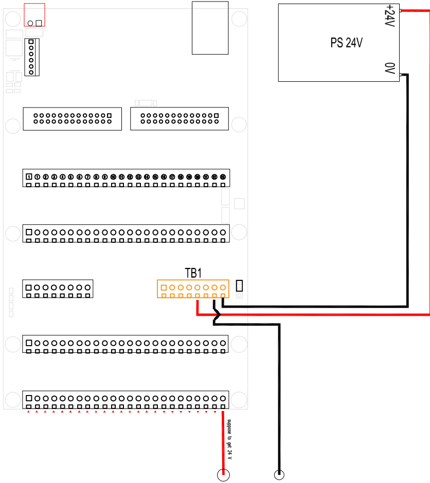
Wiring No.1
