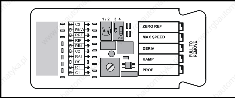
Figure 5-1 Daughter board
