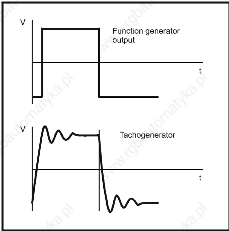
Figure 5-3 Waveform resulting from insufficient proportional gain
