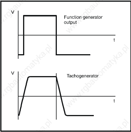
Figure 5-9 Ideal waveform
