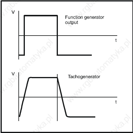
Figure 5-5 Ideal waveform
