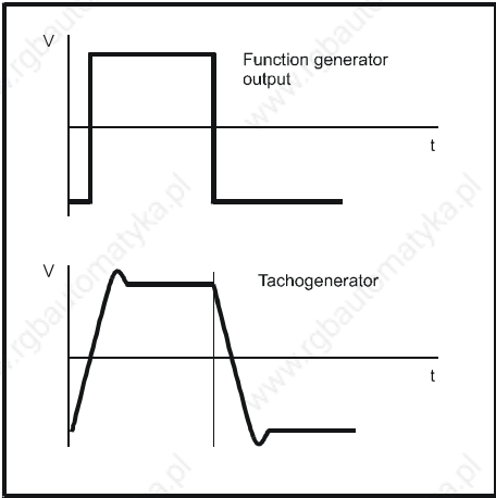
Figure 5-4 Waveform resulting from insufficient derivative gain
