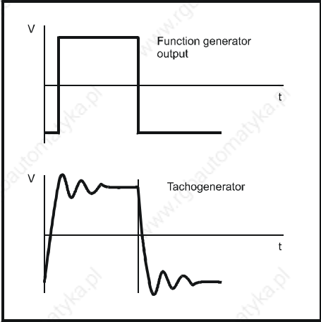
Figure 5-7 Waveform resulting from insufficient proportional gain
