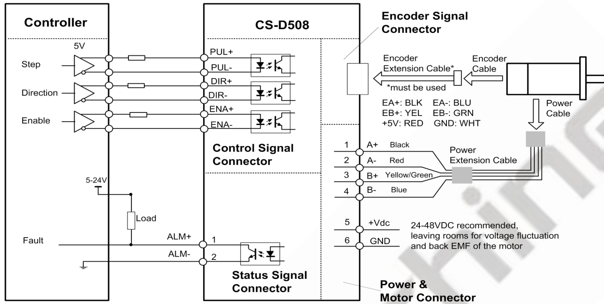
Figure 7: Typical connection
