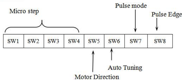
Figure 6 DIP switch Setting
